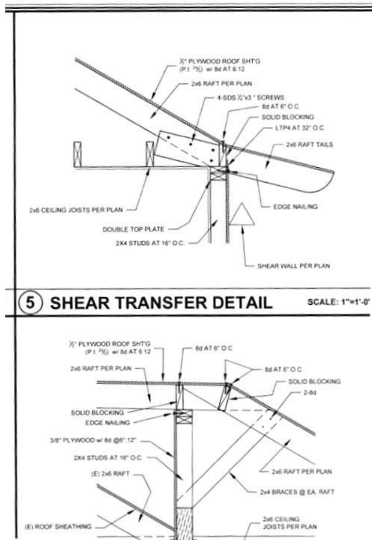
Construction detail- roof edge curve and soffit
